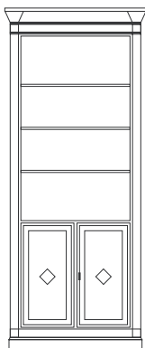
Art. 2070 Modulo Carlo X centrale 2 porte + giorno Carlo X central module 2 doors + open compartments Modul Carlo X Mittelelement, 2-türig + offene Fächer L 95 P 46 H 232 m 3 1,10
